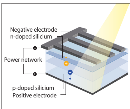
Fig.1 : Functional principle
